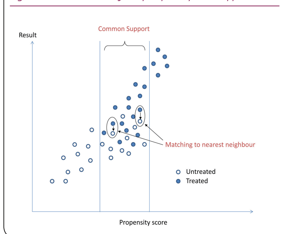
Figure 3. Illustration of the propensity score approach
